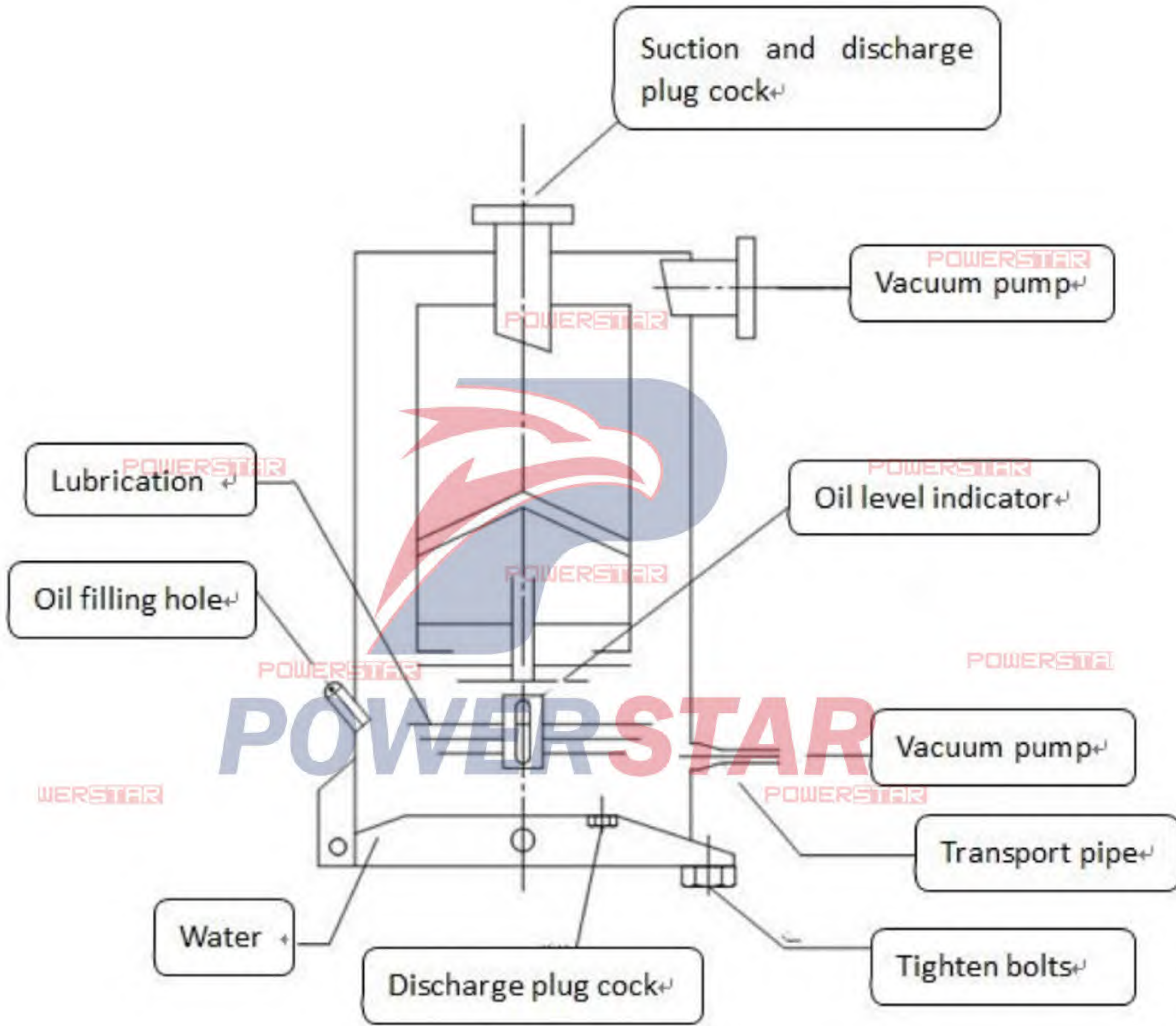
(Second Level Oil-Gas Separator)
