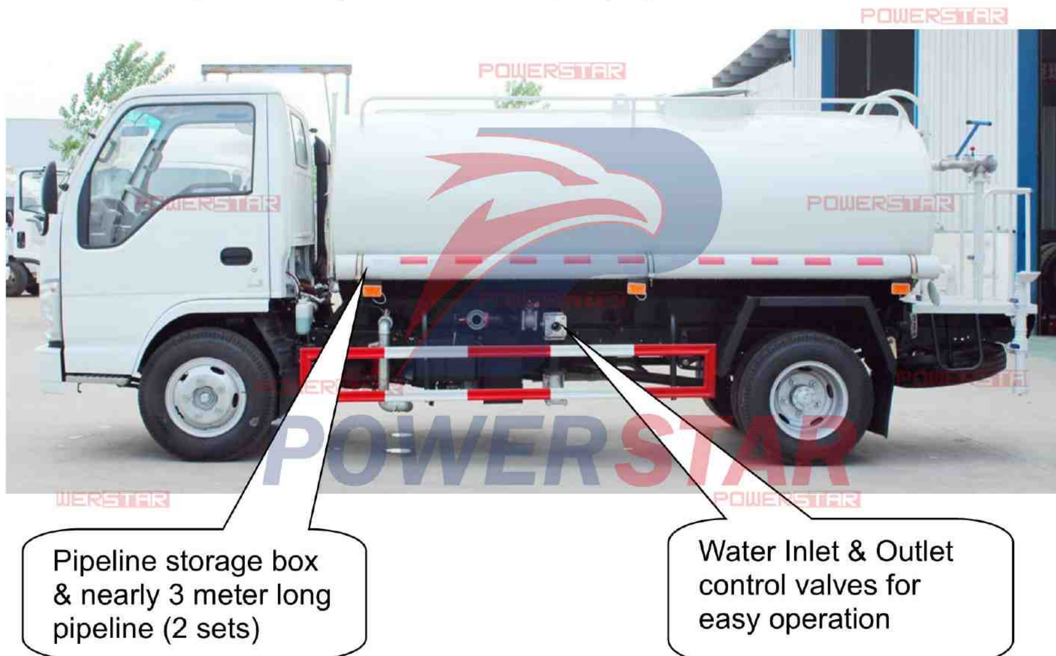
Side of the Tank: Pipeline storage box and Water pump system
